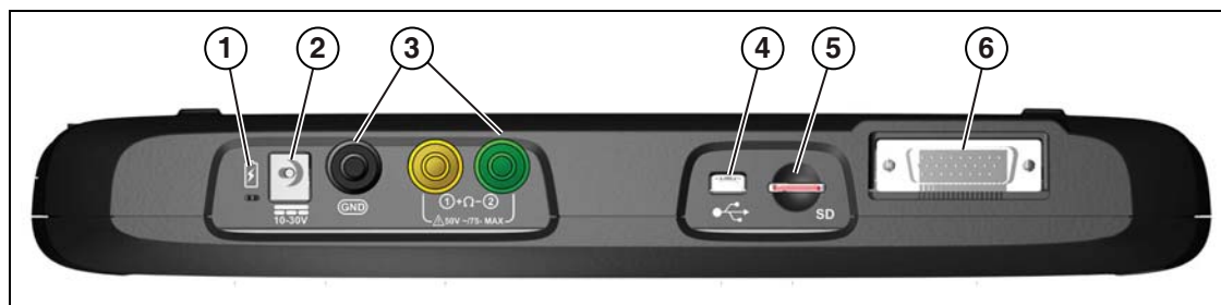
Figure 2-2 Top view
