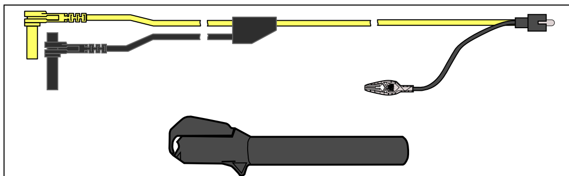
Figure 10-4 Secondary Ignition Coil Adapter Lead and Clip-on Wire Adapter
