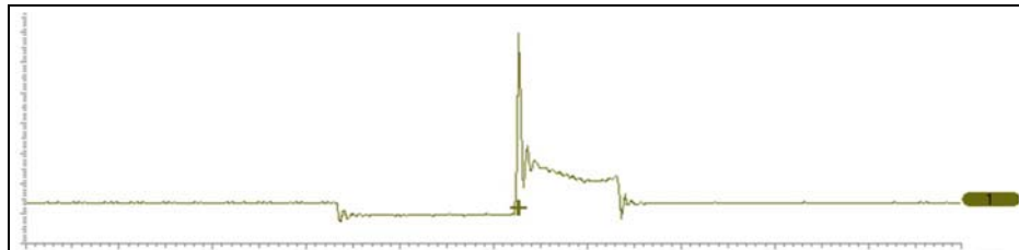
Figure 10-24 Typical Secondary Ignition Signal
