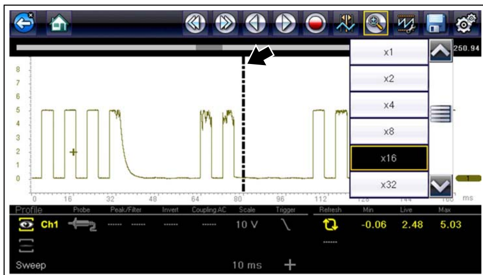
Figure 10-37 Example of Magnification Level at 16X. (For illustration purposes, the Zoom cursor has been positioned in the area near the glitches.)
